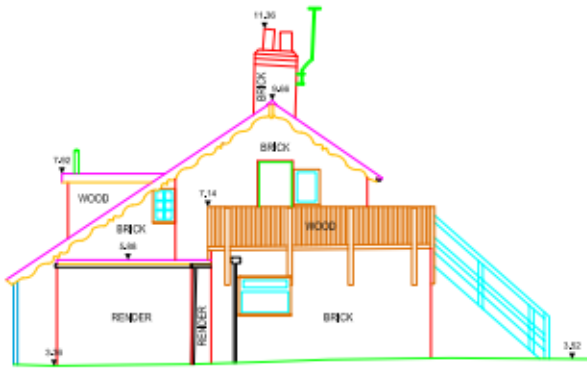
WEST ELEVATION
