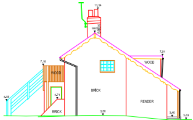
EAST ELEVATION
